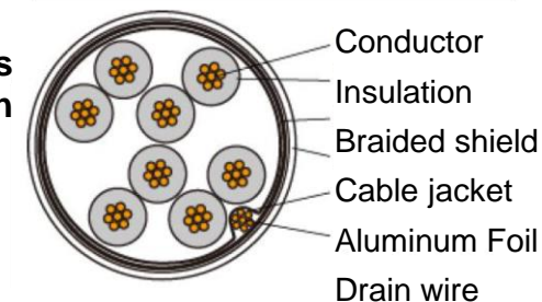
STP (Double shield structure)
