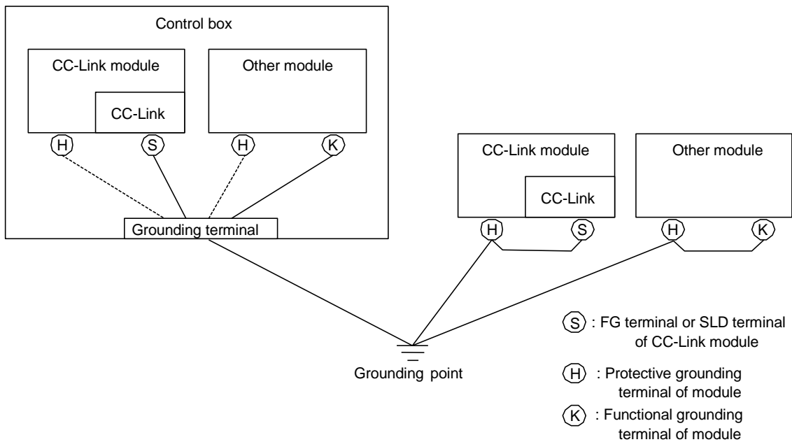
Fig. 4.8 Common grounding example
