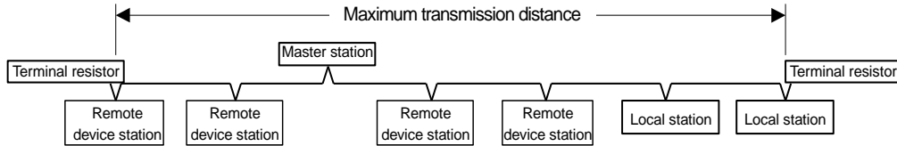
Fig. 2.1 Connection style
