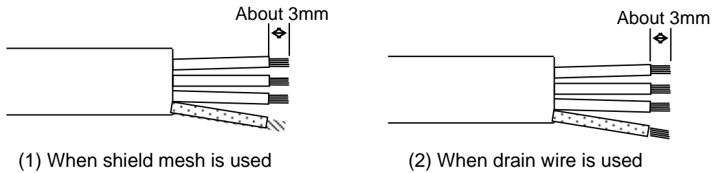
Fig. 4.3 Remove signal wire coat
